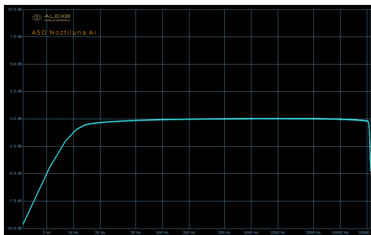
A5D-NAi frequency response (@ 0dBVU)
