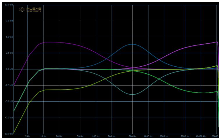
A5M-N·Ai frequency response (@ 0dBVU)
