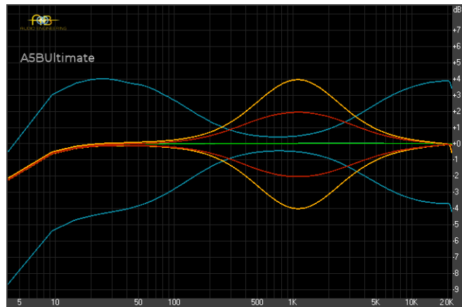
A5B frequency response (@ 0dBVU)
