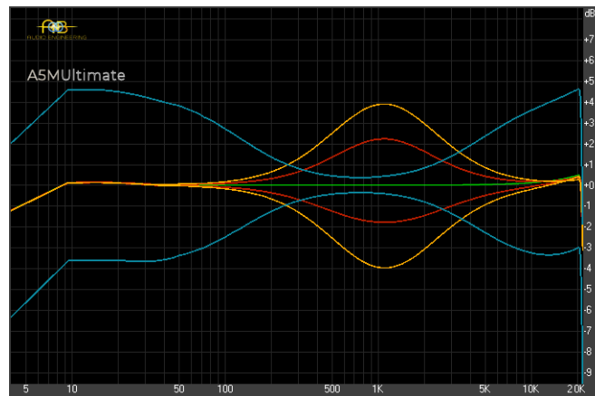
A5M frequency response (@ 0dBVU)
