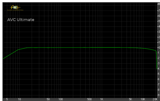
AVC frequency response (@ 0dBVU)
